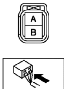
FUEL INJECTOR NO.6 WIRING HARNESS-SIDE CONNECTOR
