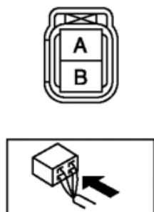
FUEL INJECTOR NO.5 WIRING HARNESS-SIDE CONNECTOR
