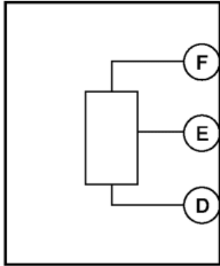
APP SENSOR WIRING HARNESS-SIDE CONNECTOR
