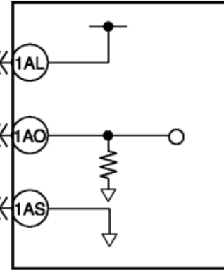
PCM WIRING HARNESS-SIDE CONNECTOR
